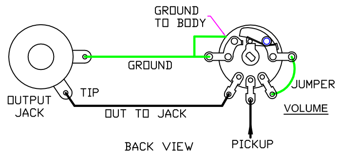
JACKPOT VOLUME CONTROL FOR PICKUP WITHOUT TONE CONTROL
